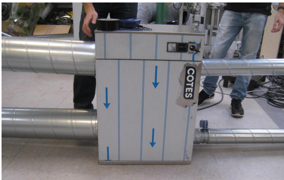
Figure 1 Test set-up for the dehumidifier C30-0.9. The front here is Position A (see Annex 1).
